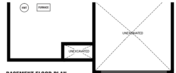
BASEMENT FLOOR PLAN ELEVATION "B"
