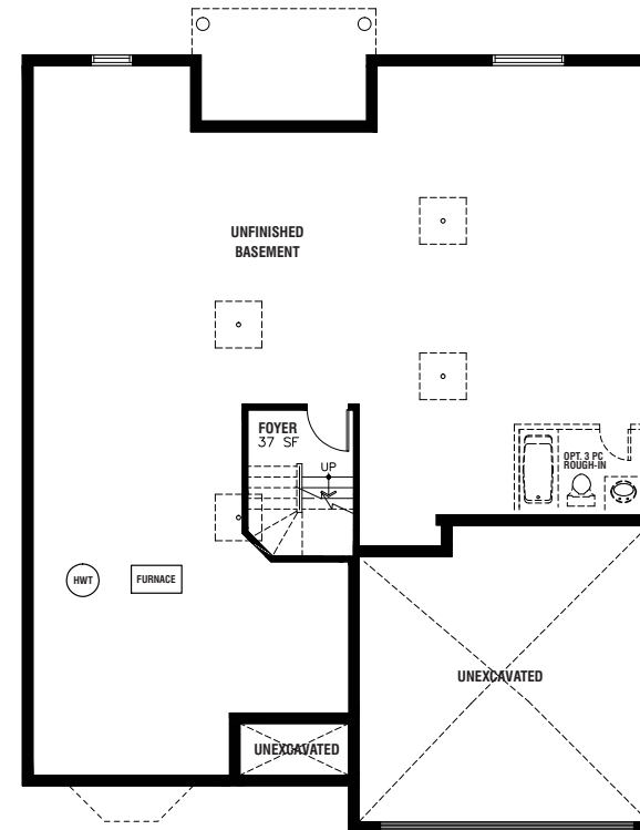
BASEMENT FLOOR PLAN ELEVATION "A"
