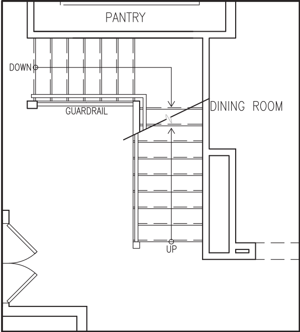
PARTIAL GROUND FLOOR PLAN
