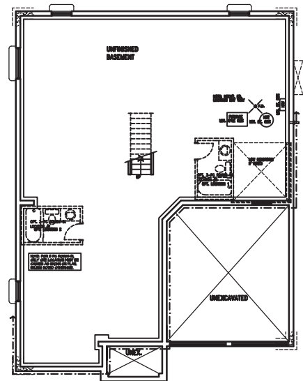
BASEMENT PLAN ELEVATION A, E
