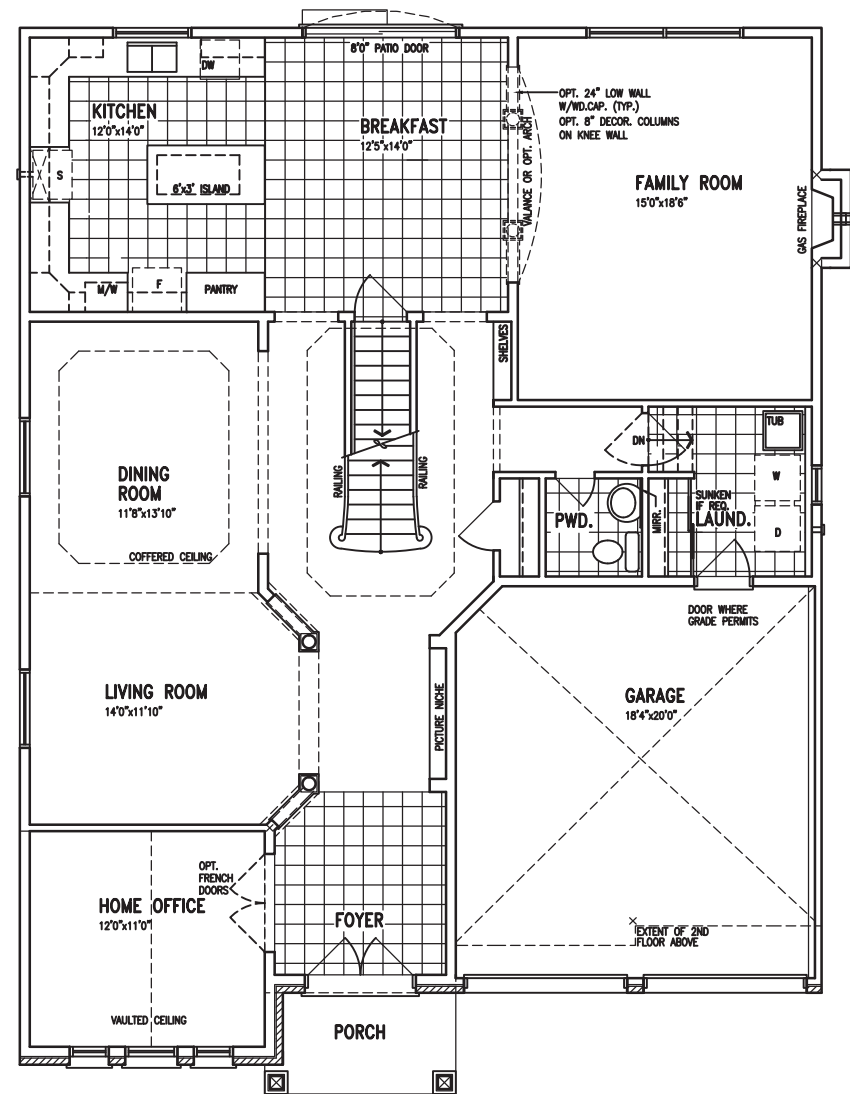
GROUND FLOOR PLAN ELEVATION A, E
