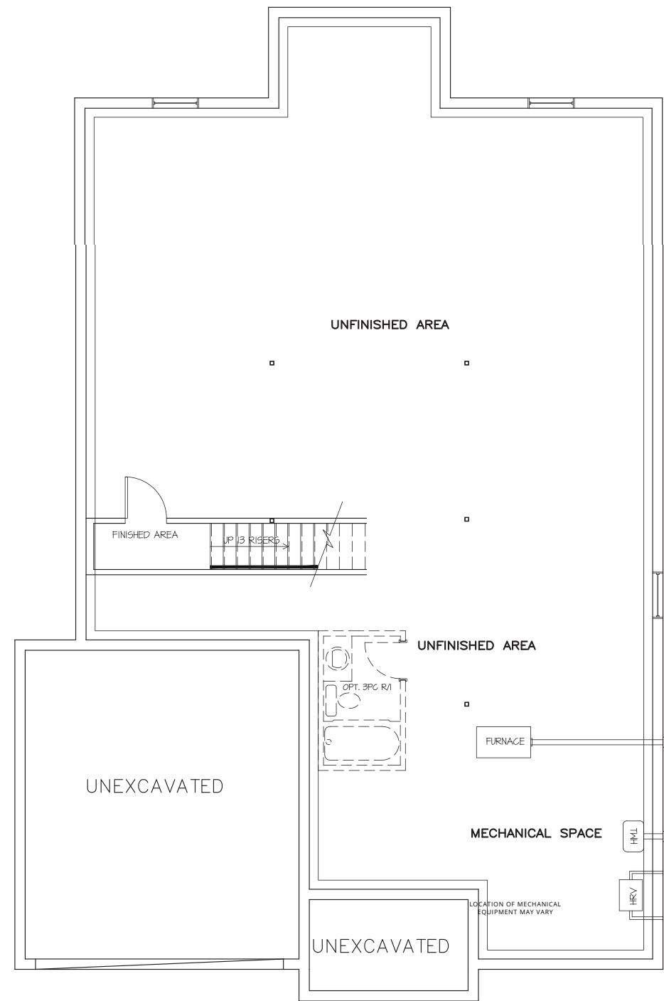
BASEMENT PLAN
