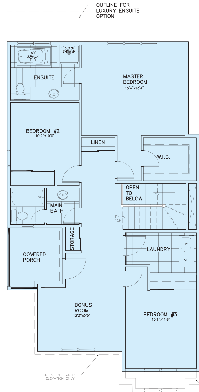
ELEVATION C/D SECOND FLOOR PLAN
