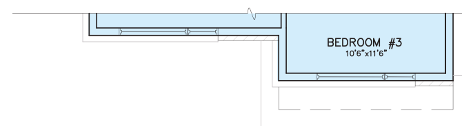
ELEVATION M SECOND FLOOR PLAN
