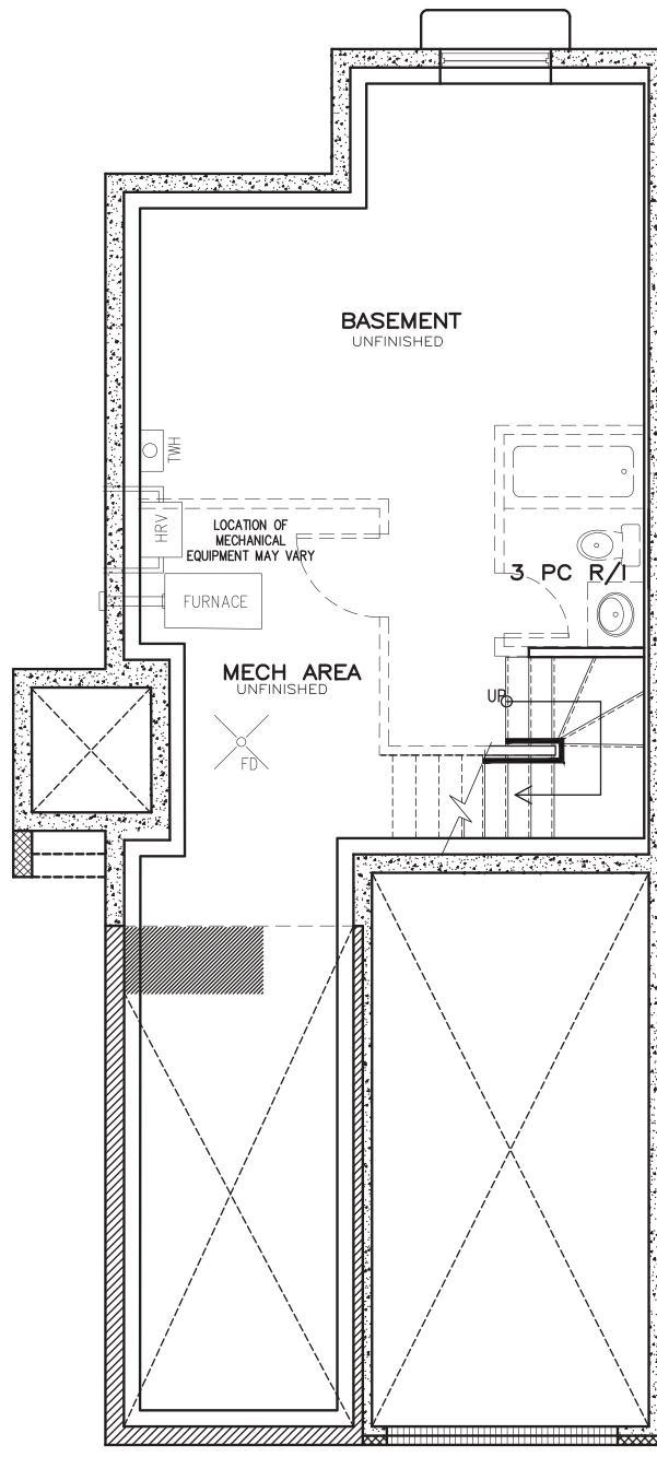
BASEMENT PLAN
