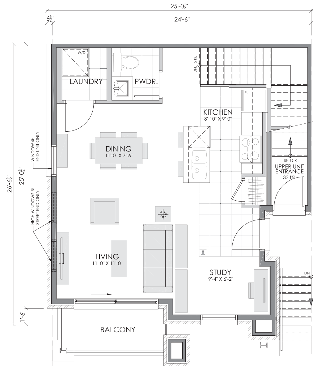
EDEN: MAIN FLOOR FLOOR AREA: 575 ff 2
