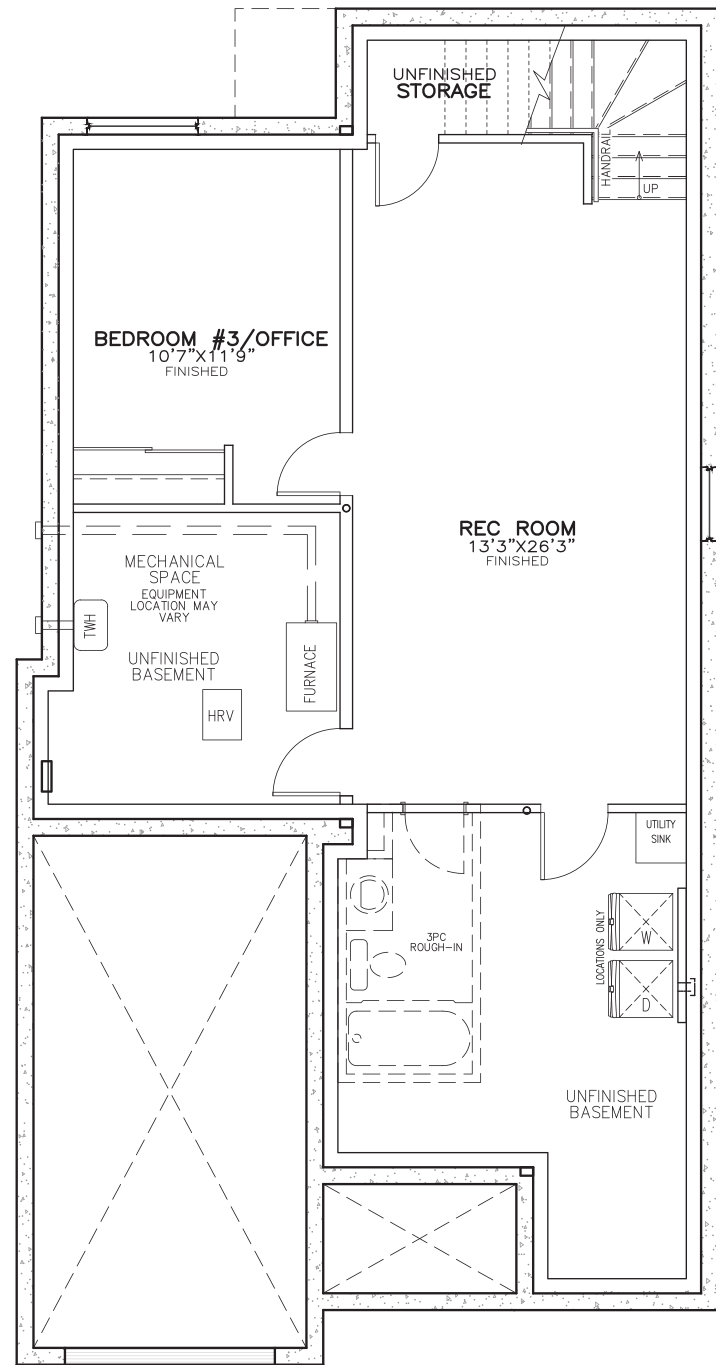
ELEVATION L FINISHED BASEMENT PLAN
