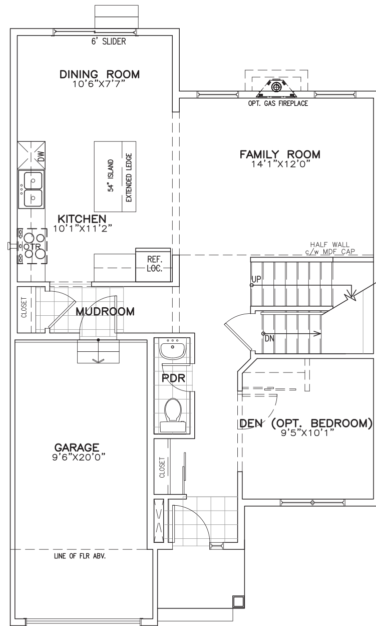
ELEVATION L GROUND FLOOR PLAN
